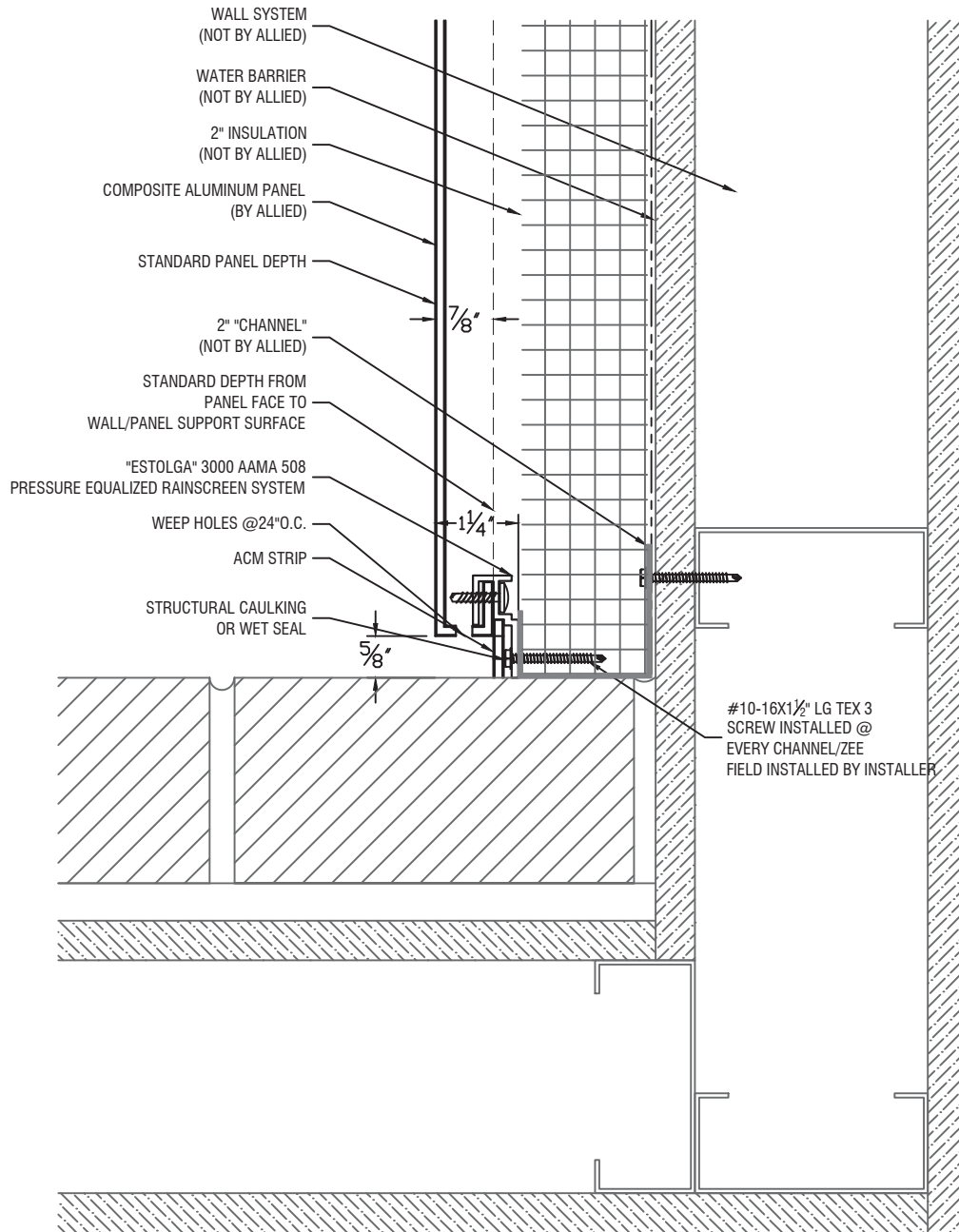
Plan Detail @ Brick Wall
